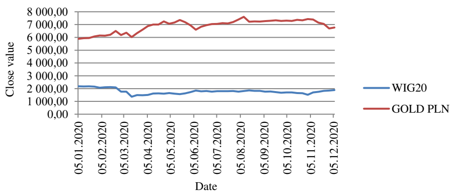
Chart 2. WIG20 and GOLD PLN in 2020 (weekly quotes)
