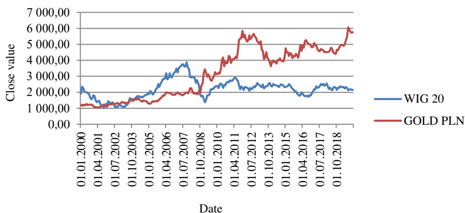
Chart 1. WIG20 and GOLD PLN in 2000–2019 (monthly quotes)
