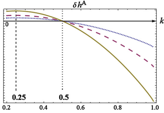
Fig. 1. The drawing qualitatively presents 3 demonstration curves (for 3 different UV cutoffs \Lambda ) of the function \delta h^A(k) defined by (20) (and (17)). For the Kasner exponents k \in (\frac{1}{4}, 1) , \delta h^A(k) is evidently decreasing function thus supporting the damping of cosmological anisotropy.
